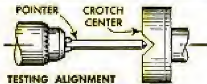
TESTING ALIGNMENT
